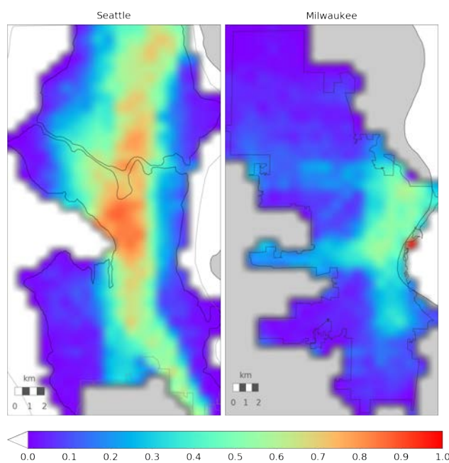
Fig. 5. Heatmaps of Seattle (left) and Milwaukee (right) showing the probability that a cell-site simulator would have been collected in the data if it were deployed at locations for a 2-hour duration with a detection radius of 1303 meters. These heatmaps correspond to the points plotted on the curves in Fig. 6.
